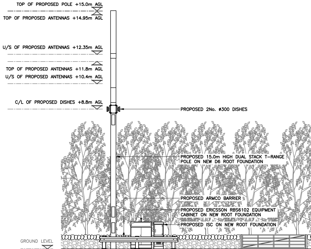
PROPOSED SOUTH EAST ELEVATION (1:100)
